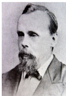
Figura 5 – Francis Guthrie
